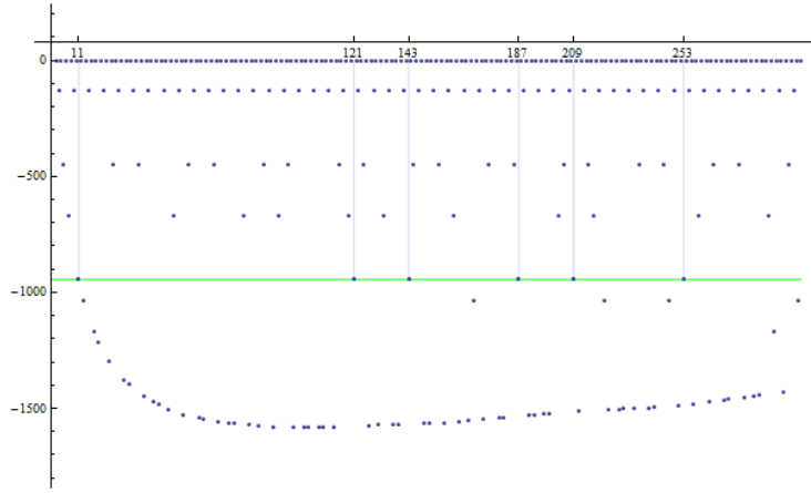
Figure 16: \log_{10} |\delta_{3001,n} - 1|
