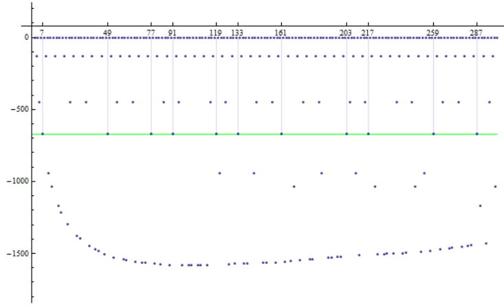
Figure 15: \log_{10} |\delta_{3001,n} - 1|
