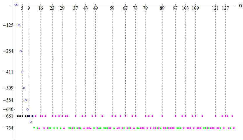
Figure 29: Modified series (91)
