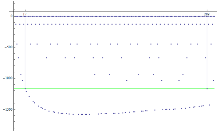
Figure 18: \log_{10} |\delta_{3001,n} - 1|
