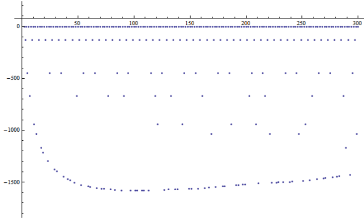
Figure 13: \log_{10} |\delta_{3001,n} - 1|
