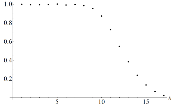
Figure 1: Coefficients \delta_{17,n}
