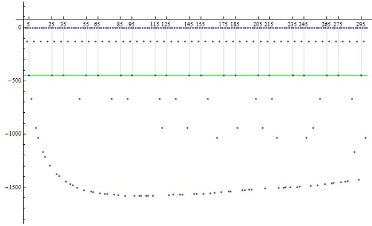
Figure 14: \log_{10} |\delta_{3001,n} - 1|
