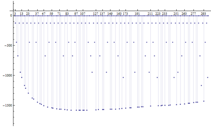
Figure 19: \log_{10} |\delta_{3001,n} - 1|
