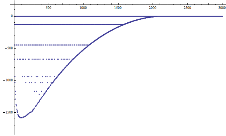
Figure 20: \log_{10} |\delta_{3001,n} - 1|
