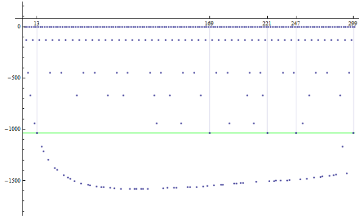
Figure 17: \log_{10} |\delta_{3001,n} - 1|
