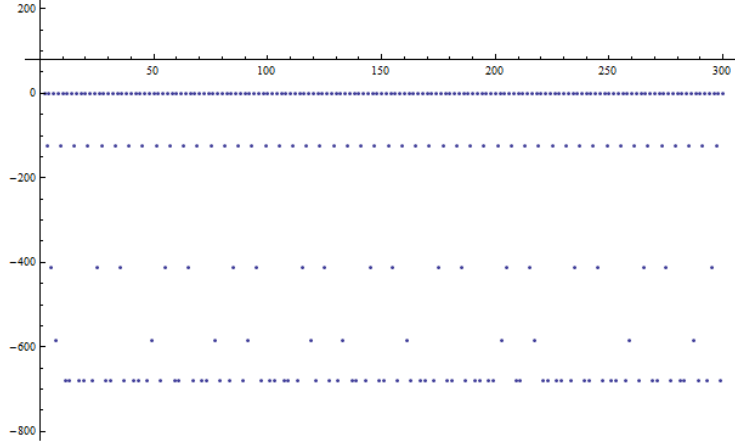
Figure 24: \log_{10}(|\delta_{3000,n}^\Gamma - 1|)
