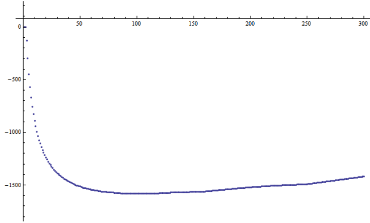
Figure 22: \log_{10} |\mu_{3001,n}|
