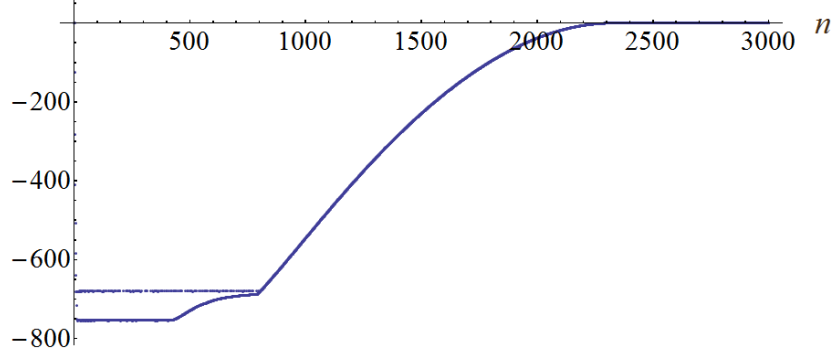
Figure 30: \log_{10} |\mu_{3000,n}^\Gamma|
