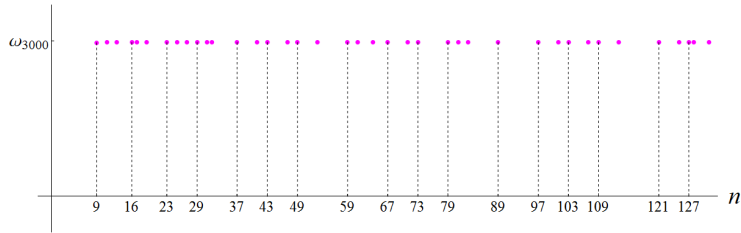
Figure 28: \frac{\mu_{3000,n}^\Gamma}{\Lambda(n)}
