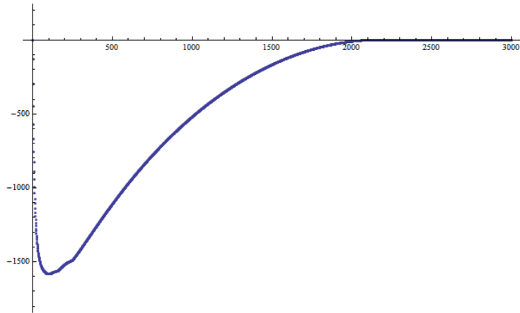
Figure 23: \log_{10} |\mu_{3001,n}|
